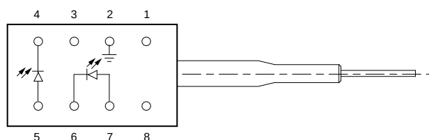
Figure 1. D370-Type Digital Uncooled Laser Module Schematic, Top View
