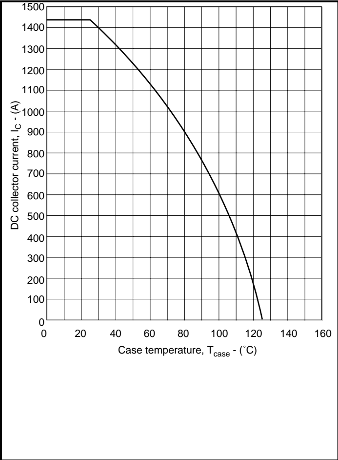
Fig. 15 DC current rating vs case temperature
