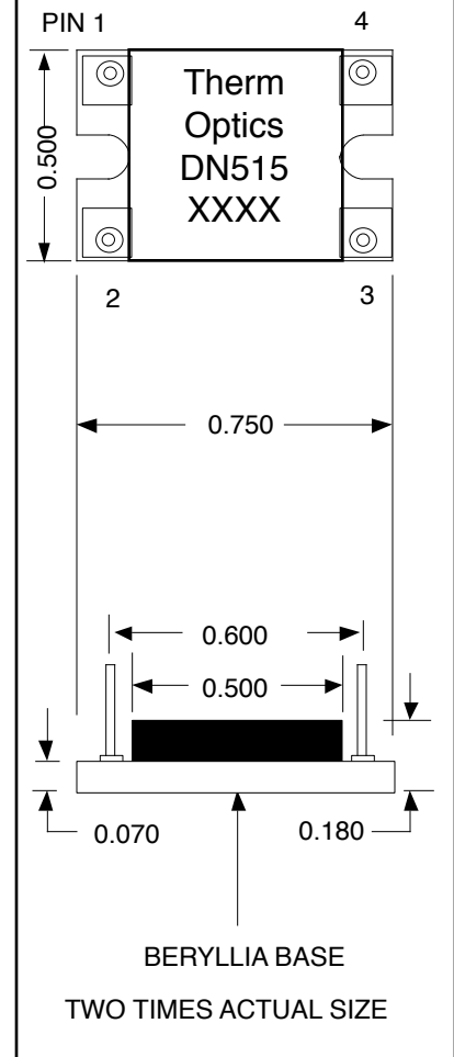
OUTLINE DIMENSIONS
