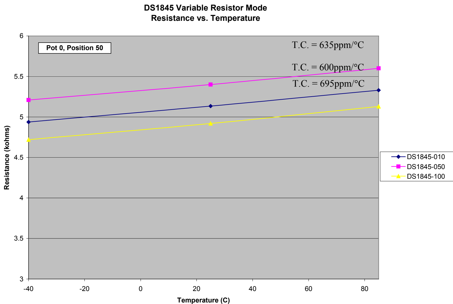
Figure 5. DS1845 in Variable Resistor Mode (Pot 0)
