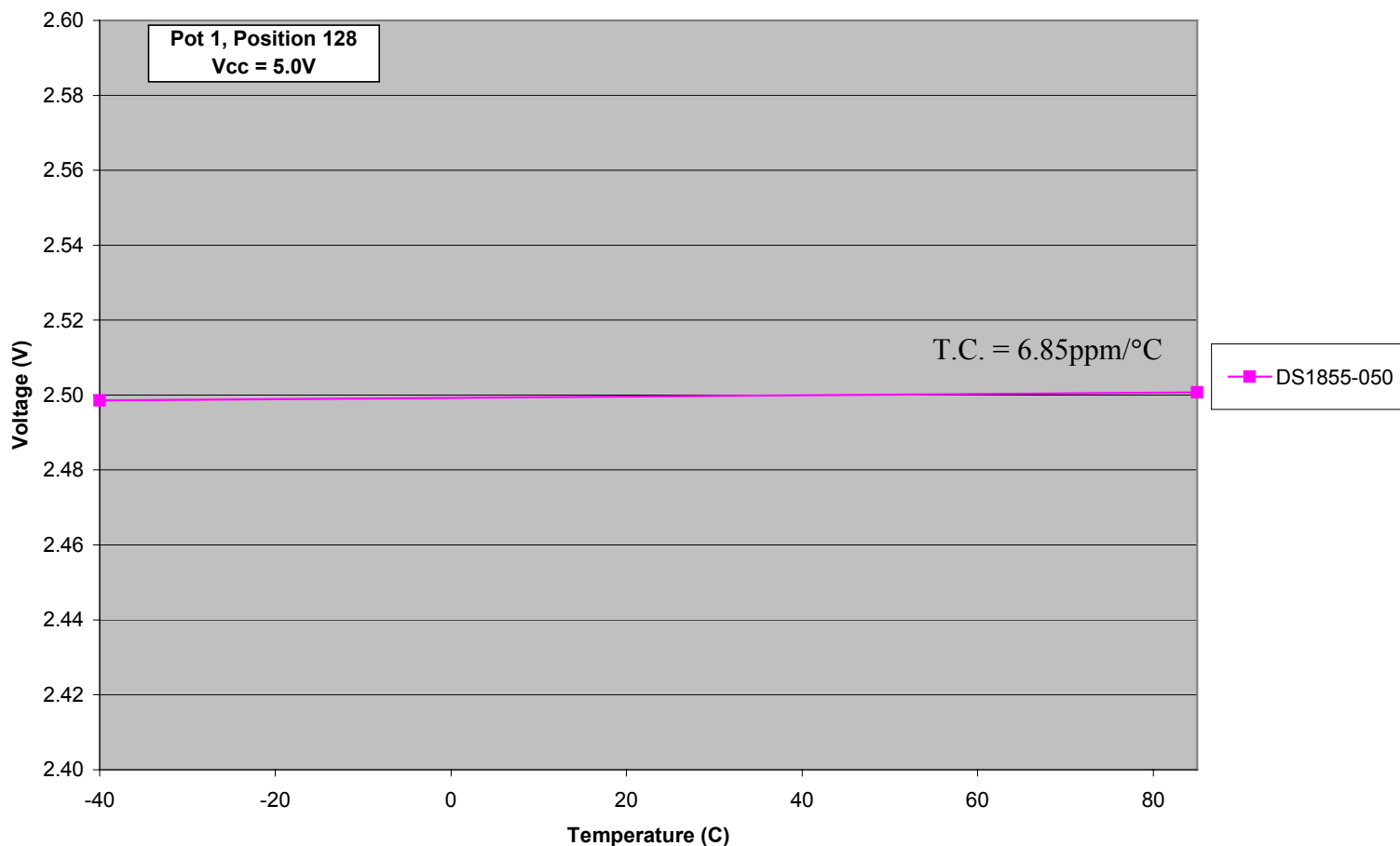
DS1855 Voltage Divider Mode Voltage vs. Temperature
