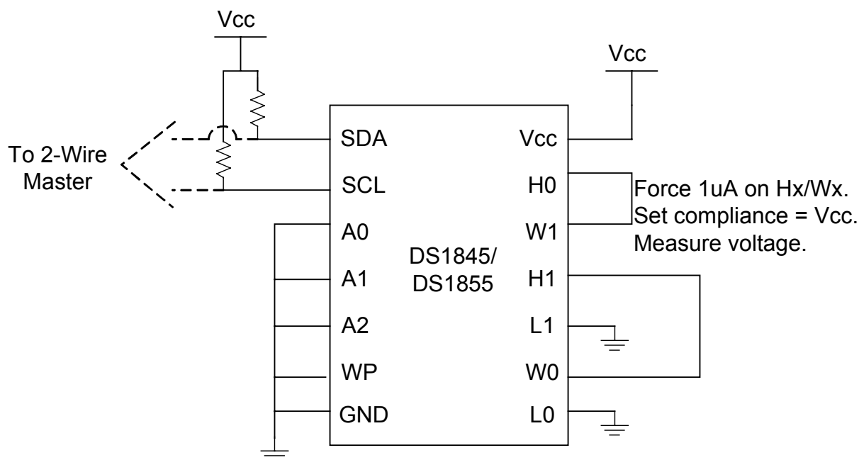
Figure 3. Variable Resistor Mode
