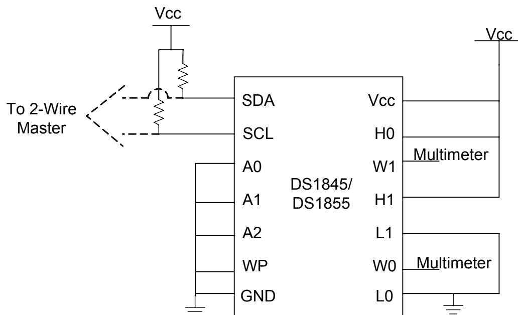
Figure 2. Voltage Divider Mode
