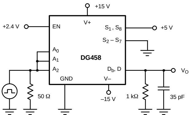
FIGURE 4. Break-Before-Make Time
