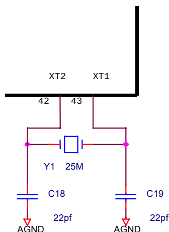
Figure 7 Crystal Circuit Diagram
