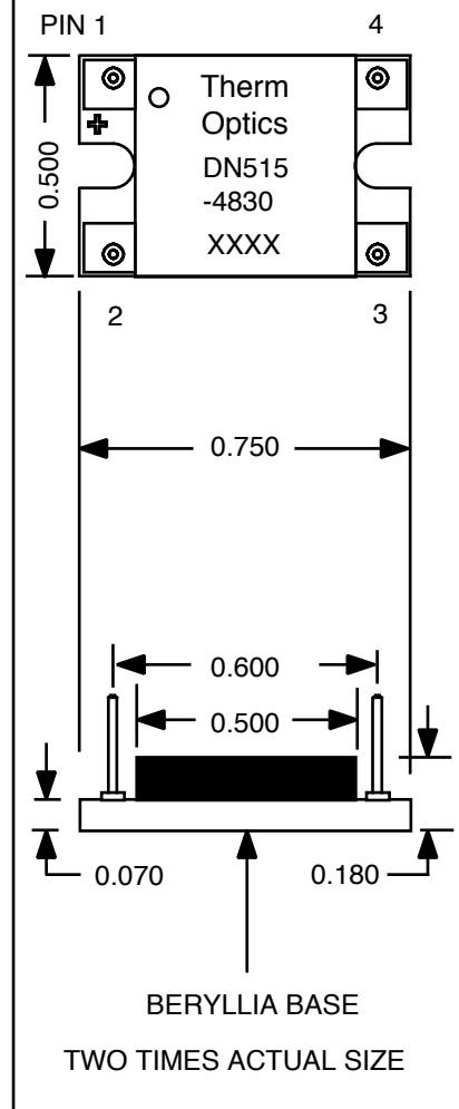
OUTLINE DIMENSIONS
