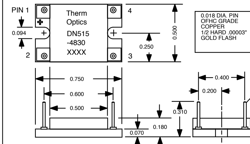
MECHANICAL DIMENSIONS
