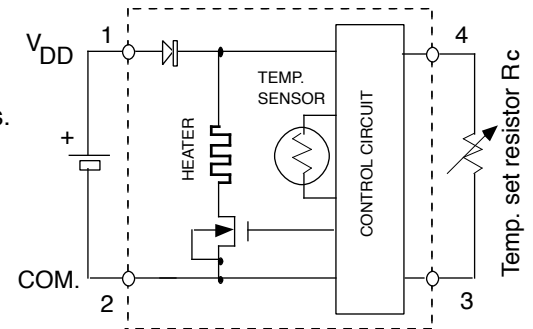
HEATER BLOCK DIAGRAM
