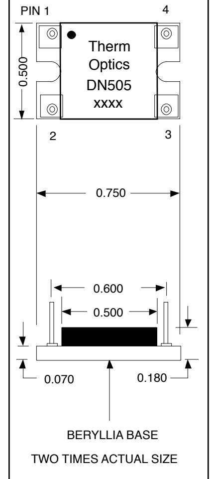
OUTLINE DIMENSIONS
