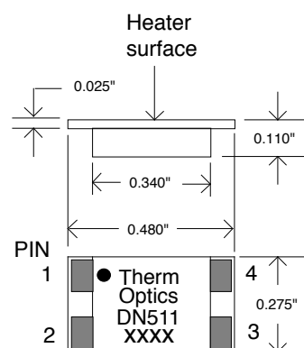
OUTLINE DIMENSIONS
