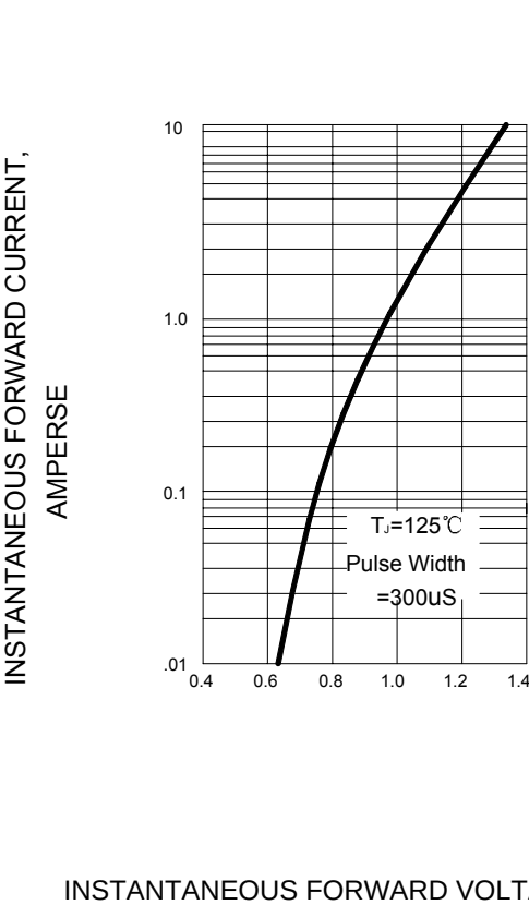
FIG.3 – TYPICAL FORWARD CHARACTERISTIC
