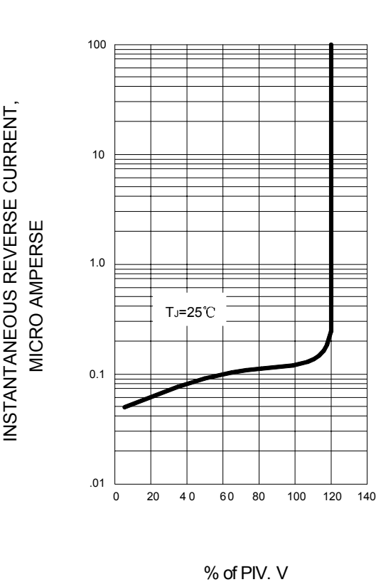
FIG.4 – TYPICAL REVERSE CHARACTERISTIC
