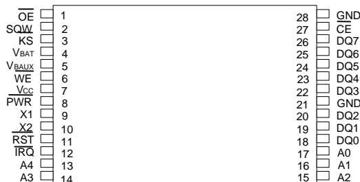
28-Pin TSOP
