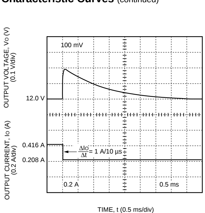
Figure 5. DC025 Dual-Output-Series Typical 12 V Output Voltage Response to a Step Load Change from 50% to 25% of I_{o,max} at V_i = V_{i,nom} and T_c = 25^\circ\text{C}
