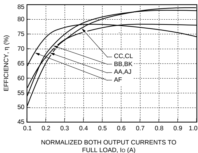
Figure 3. DW025-Series Efficiency vs. Normalized Both Output Currents to Full Load at V_I = 48\text{ V} and T_A = 25^\circ\text{C}
