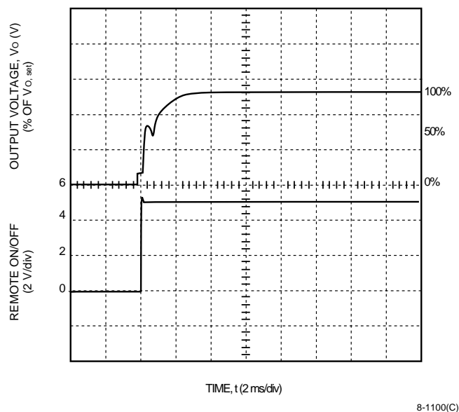
Figure 17. DW025 Triple Output-Series Typical Output Voltage Start-Up when Signal Applied to Remote On/Off
