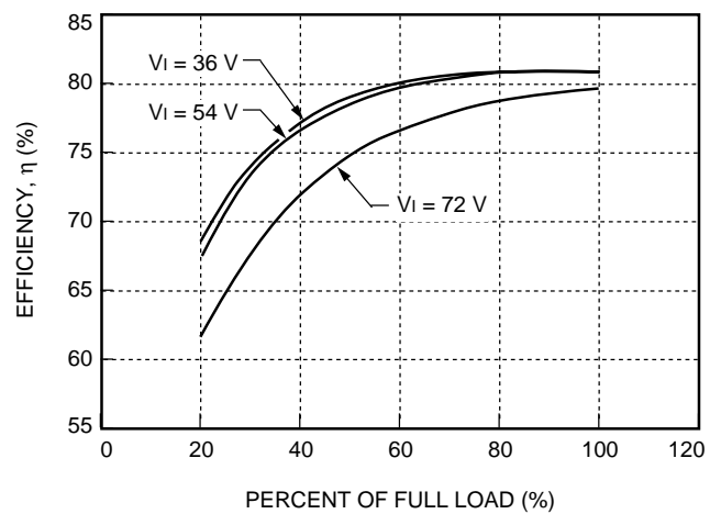
Figure 12. DW025ACL-M Typical 15 V Output Characteristics
