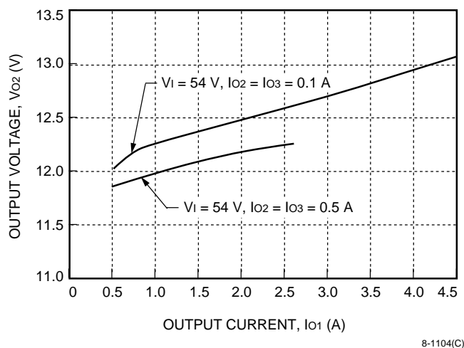
Figure 6. DW025ABK-M Typical Cross Regulation with Respect to I_{01}
