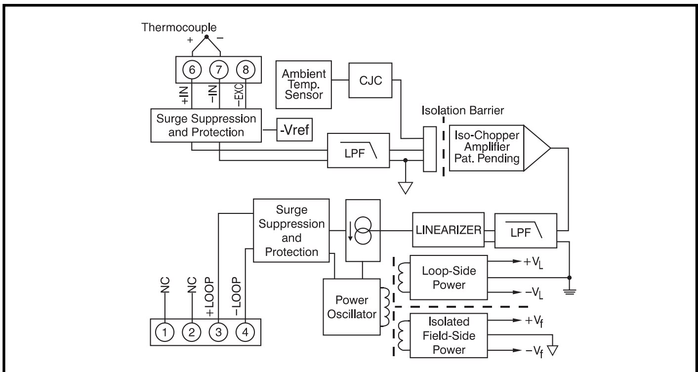
Figure 1: DSCT47 Block Diagram
