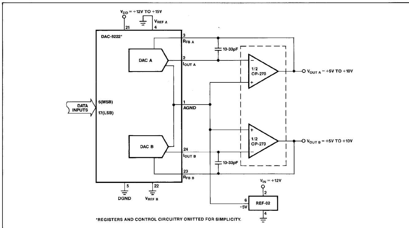
FIGURE 7: Single Supply Operation (Current Steering Mode)
