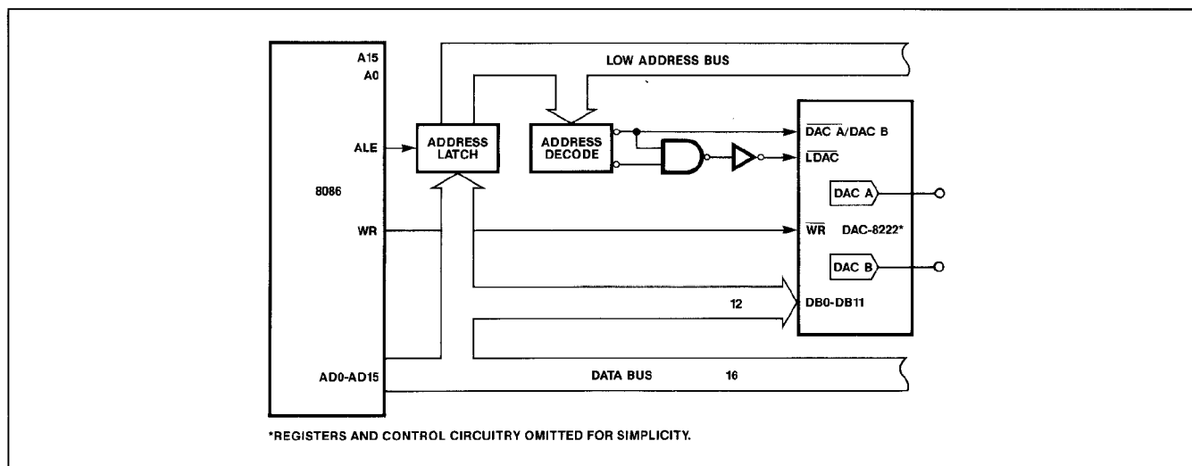
FIGURE 10: DAC-8222 To 8086 Interface
