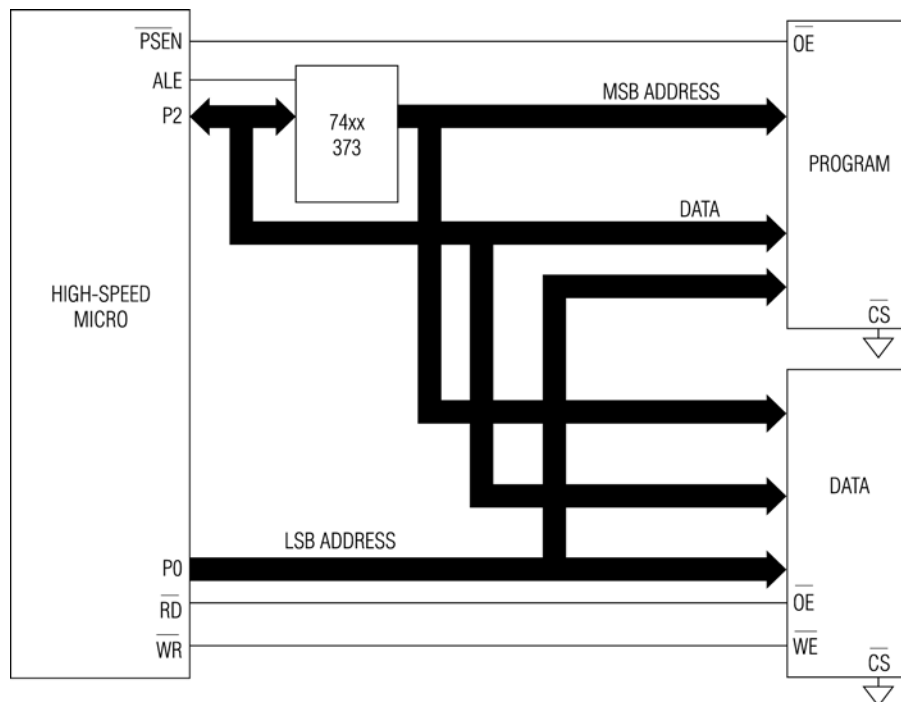
Figure 3. PAGE MODE 2 MEMORY INTERFACE
