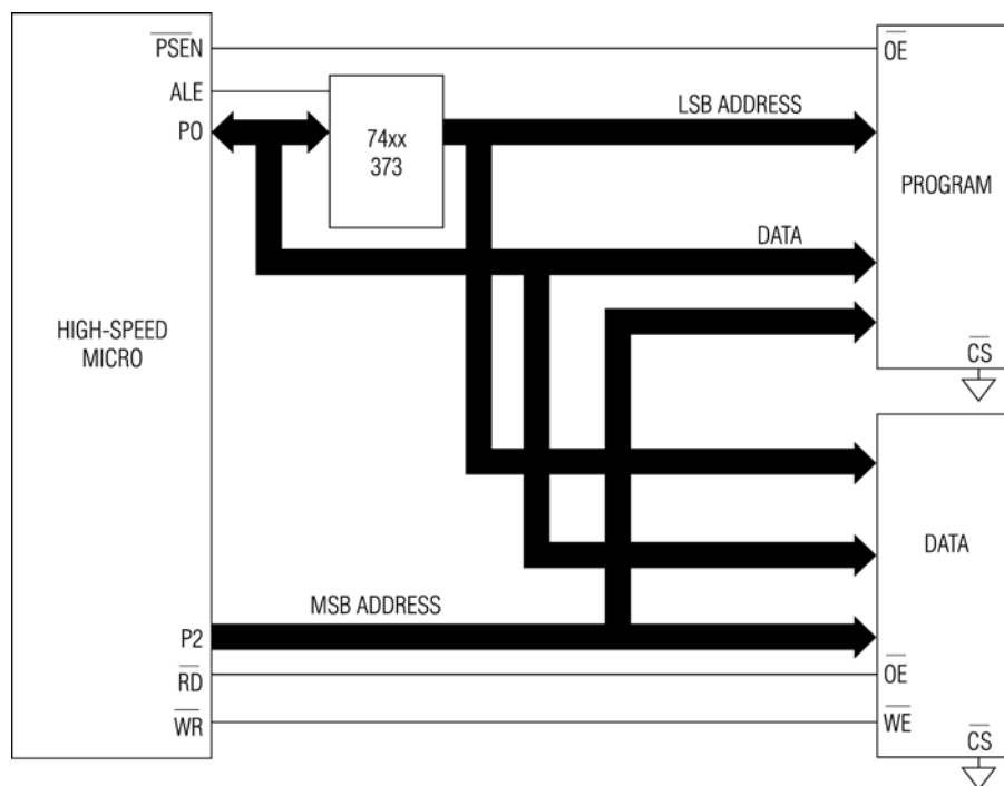
Figure 1. NON-PAGE MODE MEMORY INTERFACE
