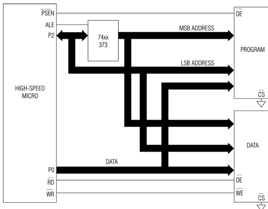
Figure 2. PAGE MODE 1 MEMORY INTERFACE
