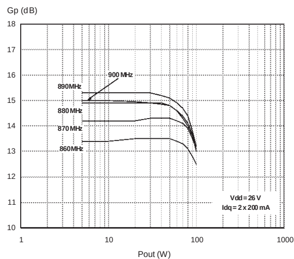
Power Gain vs. Input Power
