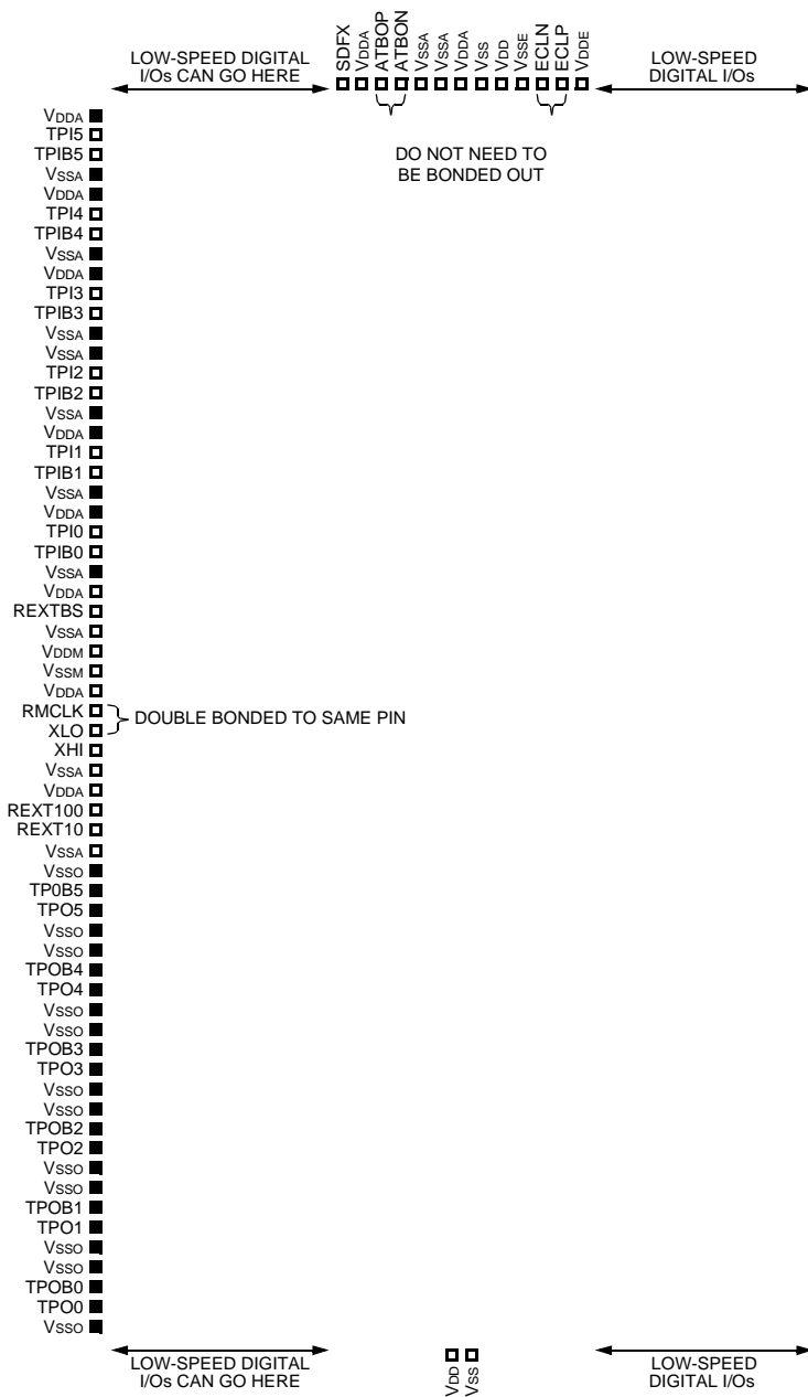
Figure 7. Pinout Assignment
