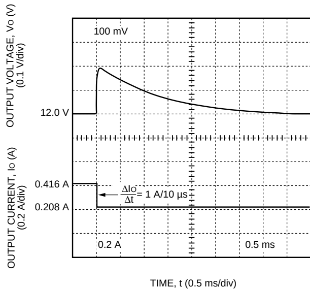
Figure 5. Typical DW025-Series 12 V Output Voltage Response to a Step Load Change from 50% to 25% of I_{o,max} at V_i = V_{i,nom} and T_A = 25^\circ\text{C}
