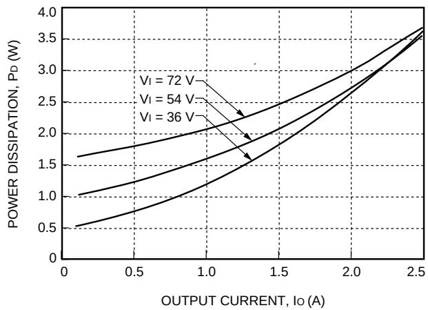
Figure 17. 5 V Output Power Dissipation vs. Output Current
