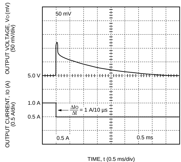
Figure 4. DW025-Series Typical 5 V Output Voltage Response to a Step Load Change from 50% to 25% of I_{O,max} at V_i = V_{i,nom} and T_A = 25^\circ\text{C}
