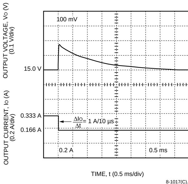
Figure 6. Typical DW025-Series 15 V Output Voltage Response to a Step Load Change from 50% to 25% of I_{o,max} at V_i = V_{i,nom} and T_A = 25^\circ\text{C}
