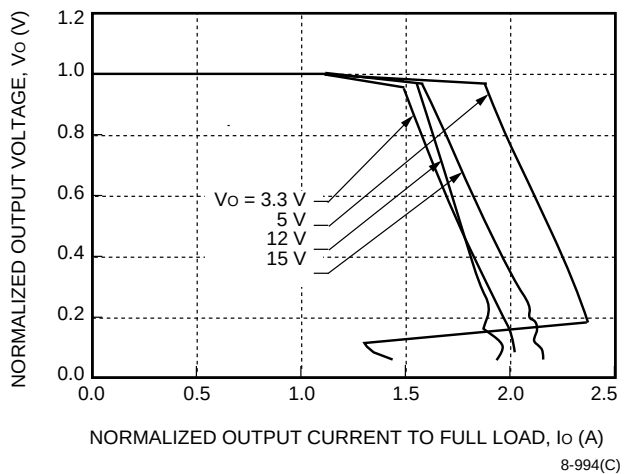
Figure 2. DW025-Series Normalized Output Current vs. Normalized Output Voltage at V_i = 48\text{ V} and T_A = 25^\circ\text{C}
