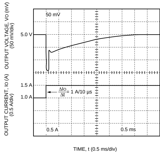
Figure 7. Typical DW025-Series 5 V Output Voltage Response to a Step Load Change from 50% to 75% of I_{o,max} at V_i = V_{i,nom} and T_A = 25^\circ\text{C}
