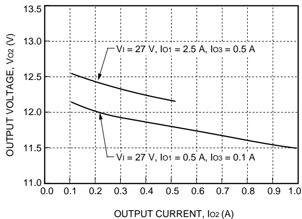
Figure 5. DC025ABK-M Typical Load Regulation
