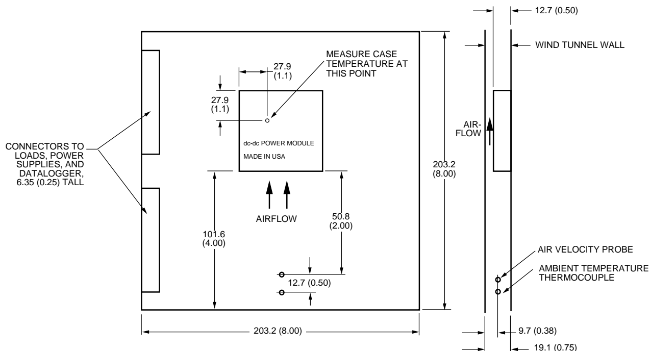
Figure 22. Thermal Test Setup
