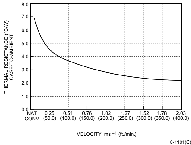
Figure 29. Case-to-Ambient Thermal Resistance vs. Air Velocity
