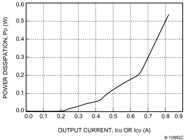
Figure 27. DC025ACL-M Losses Associated with ±15 V Output, Ps2/Ps3
