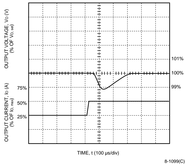
Figure 16. DC025 Triple Output-Series Typical Output Voltage for a Step Load Change from 25% to 50% of Full Load on Output 1
