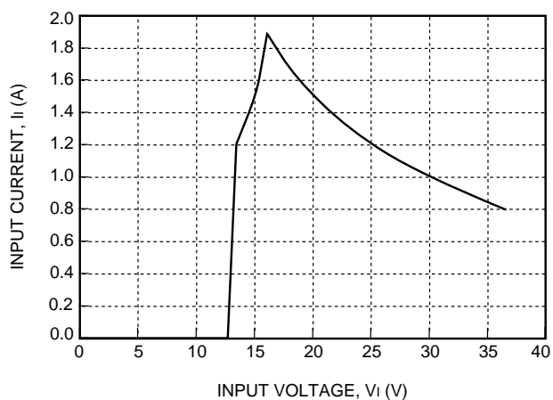
Figure 1. DC025 Triple Output-Series Typical Input Characteristics
