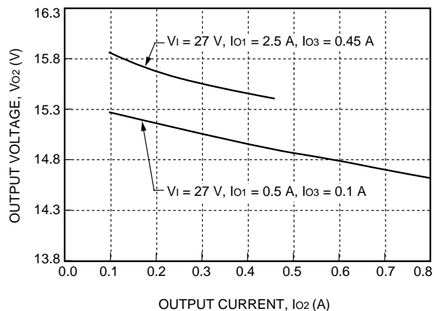
Figure 7. DC025ACL-M Typical Load Regulation
