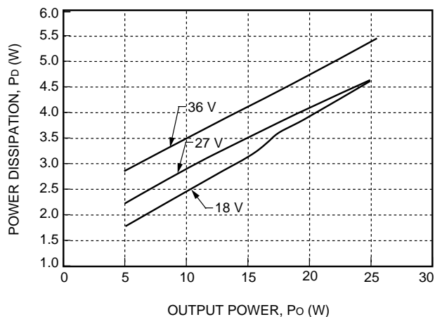
Figure 23. DC025ABK-M Fixed Losses, P_p
