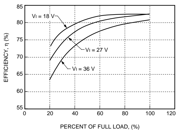
Figure 12. DC025ACL-M Typical 15 V Output Characteristics
