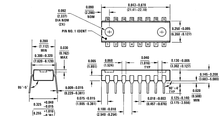
Molded Dual-in-Line Package (N) Order Number DS3245N NS Package Number N16A
