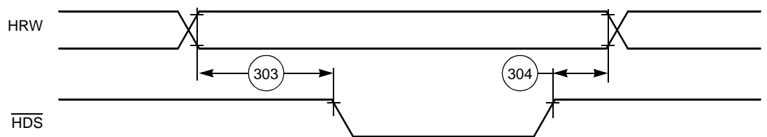
Figure 2-29. HRW to \overline{\text{HDS}} Timing
