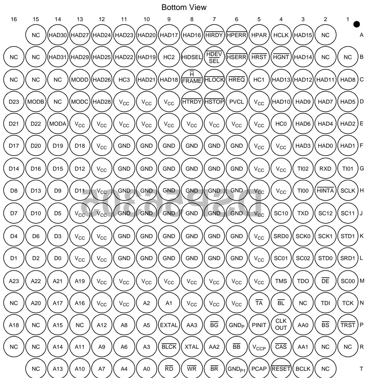
Figure 3-2. DSP56305 Molded Array Process-Ball Grid Array (MAP-BGA), Bottom View
