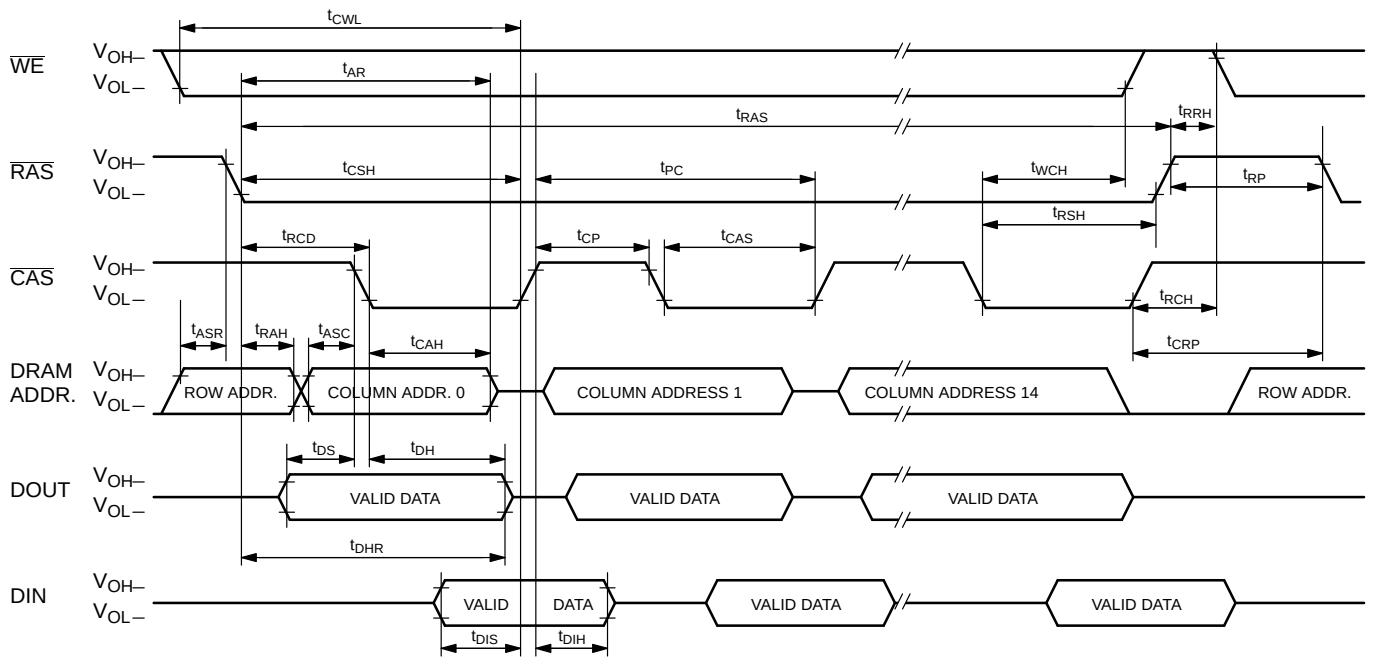
Fig. 9-14: DRAM waveform
