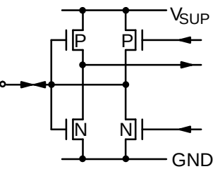
Fig. 9-8: Input/Output Pins 1 and 50
