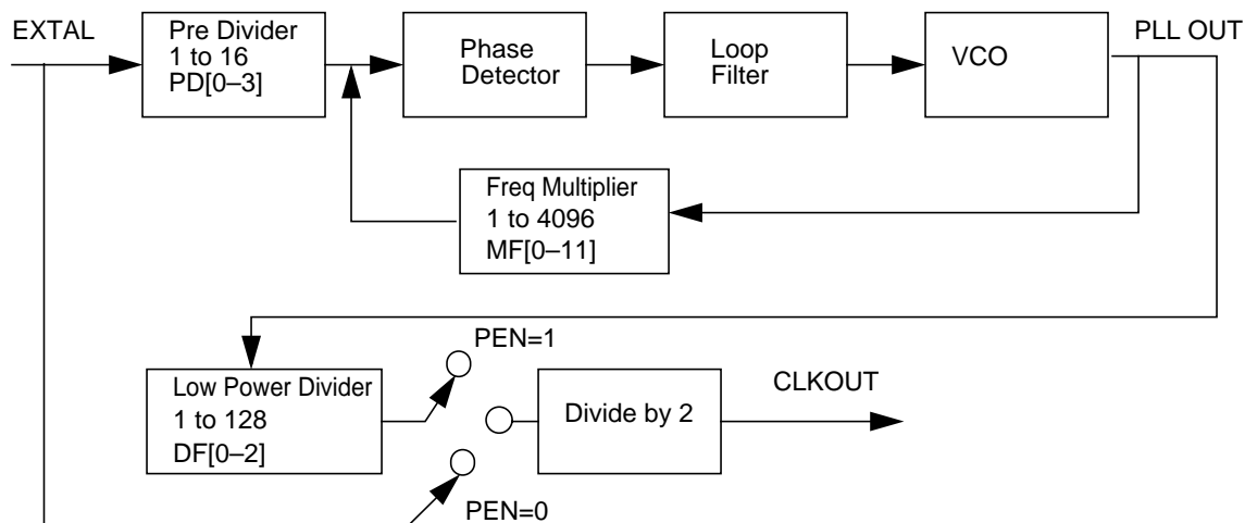
DSP56303 PLL Block Diagram
