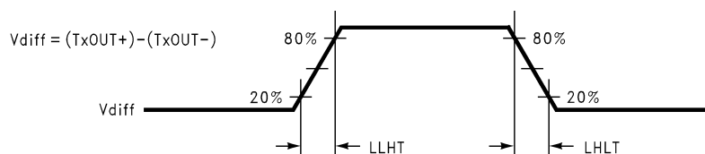
FIGURE 3. DS90CF561 (Transmitter) LVDS Output Load and Transition Timing
