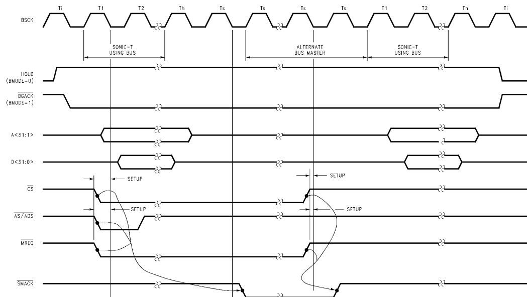
FIGURE 7-23. On-Chip Memory Arbitrator
