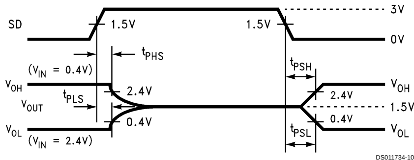
FIGURE 8. Receiver SHUTDOWN (SD) Delay Timing
