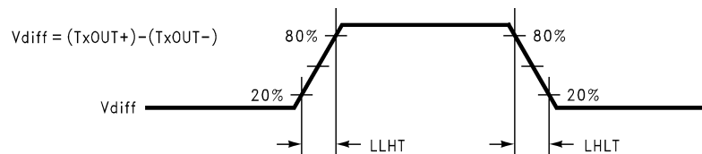
FIGURE 2. DS90CR213 (Transmitter) LVDS Output Load and Transition Times
