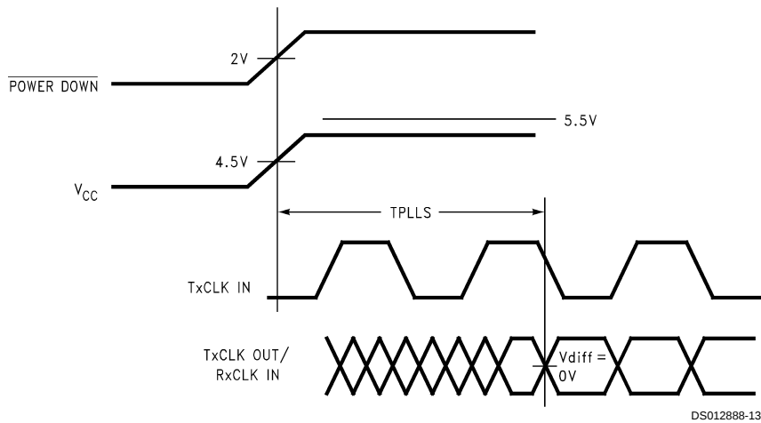
FIGURE 10. DS90CR213 (Transmitter) Phase Lock Loop Set Time
