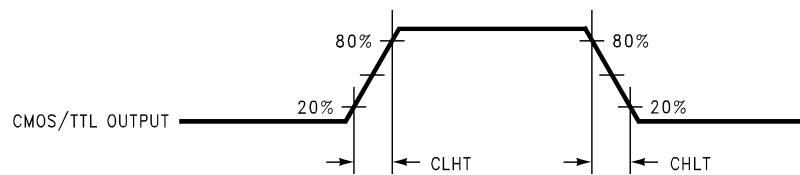
FIGURE 3. DS90CR214 (Receiver) CMOS/TTL Output Load and Transition Times
