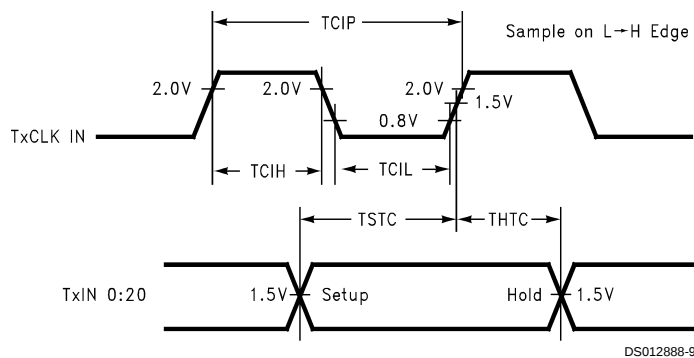
FIGURE 6. DS90CR213 (Transmitter) Setup/Hold and High/Low Times
