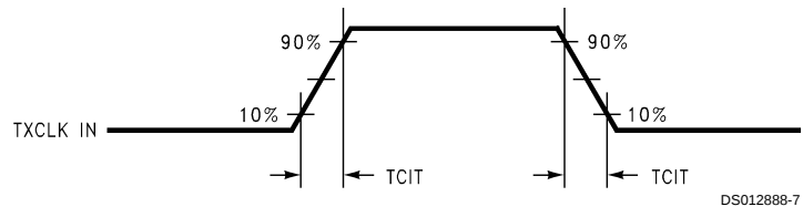
FIGURE 4. DS90CR213 (Transmitter) Input Clock Transition Time
