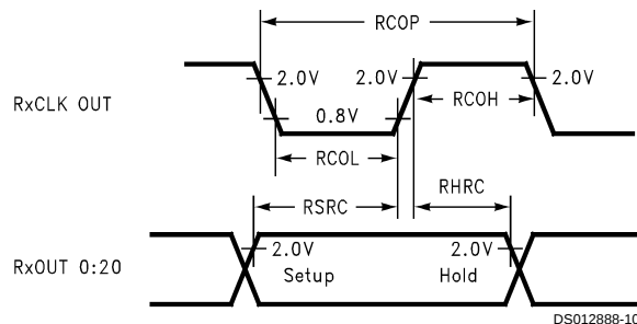
FIGURE 7. DS90CR214 (Receiver) Setup/Hold and High/Low Times
