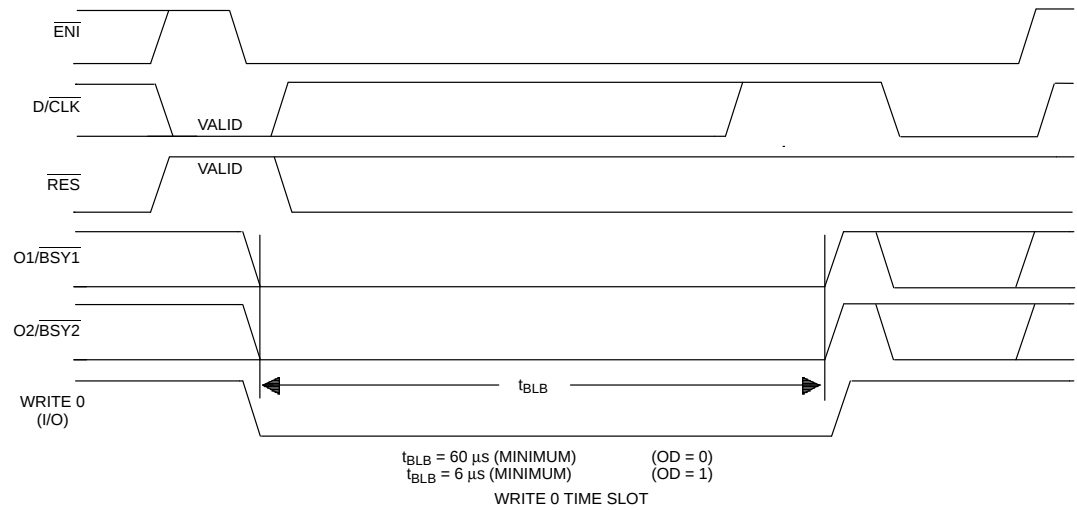
TIMING DIAGRAM: HOST INTERFACE Figure 5
