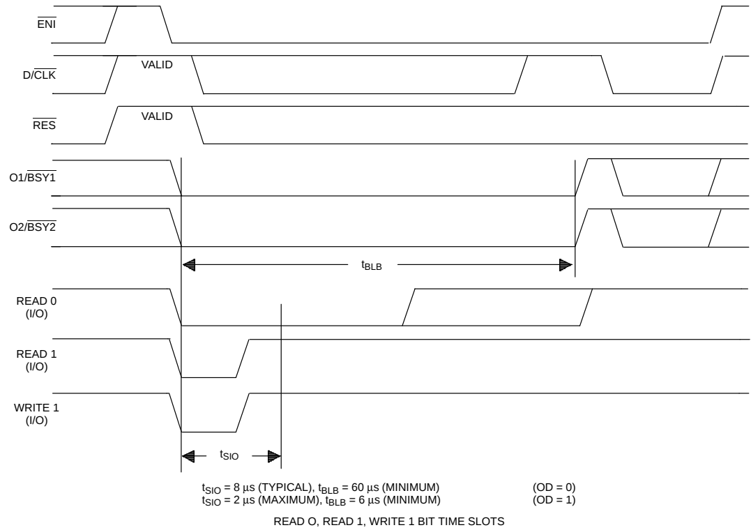
TIMING DIAGRAM: HOST INTERFACE Figure 4
