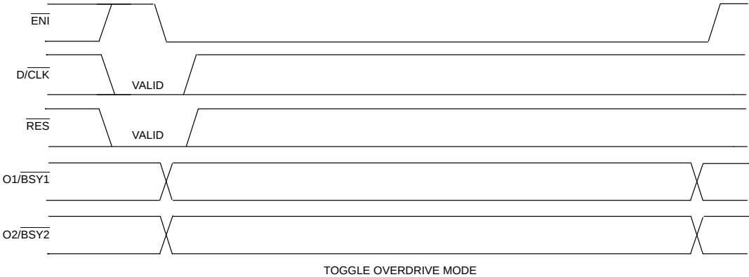
TIMING DIAGRAM: HOST INTERFACE Figure 7
