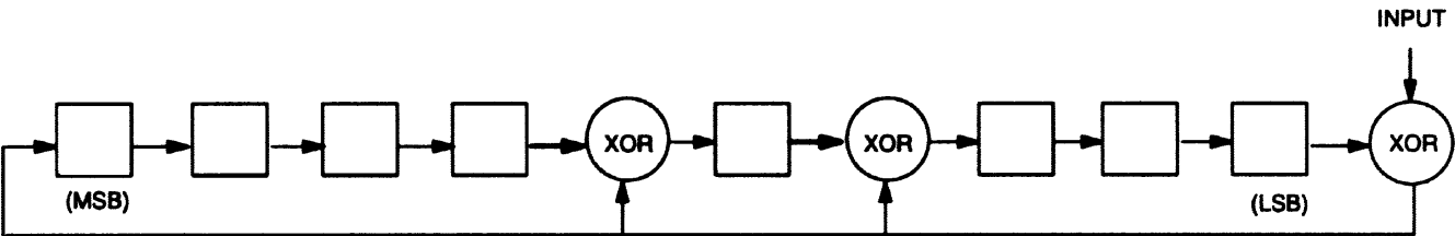
1-WIRE CRC CODE Figure 3
