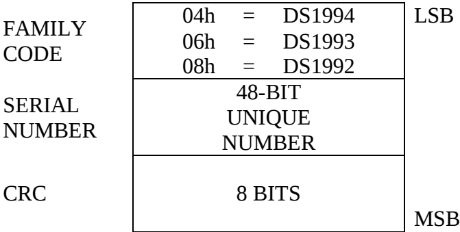
64-BIT LASERED ROM Figure 2
