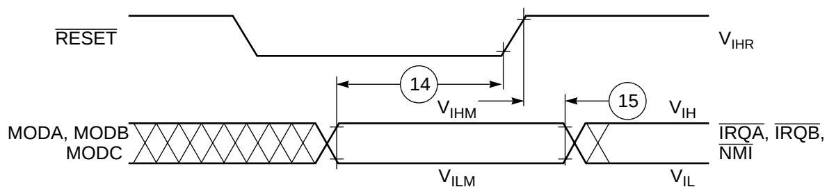
Figure 2-3 Operating Mode Select Timing
