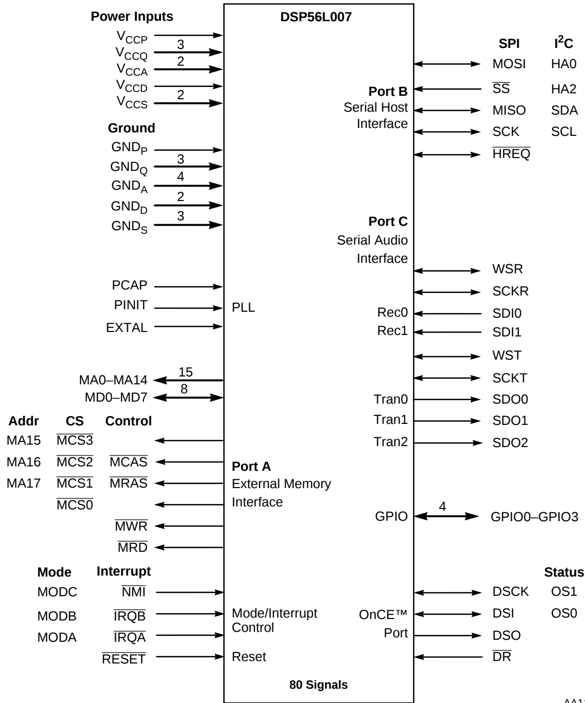
Figure 1-1 DSP56L007 Signals
