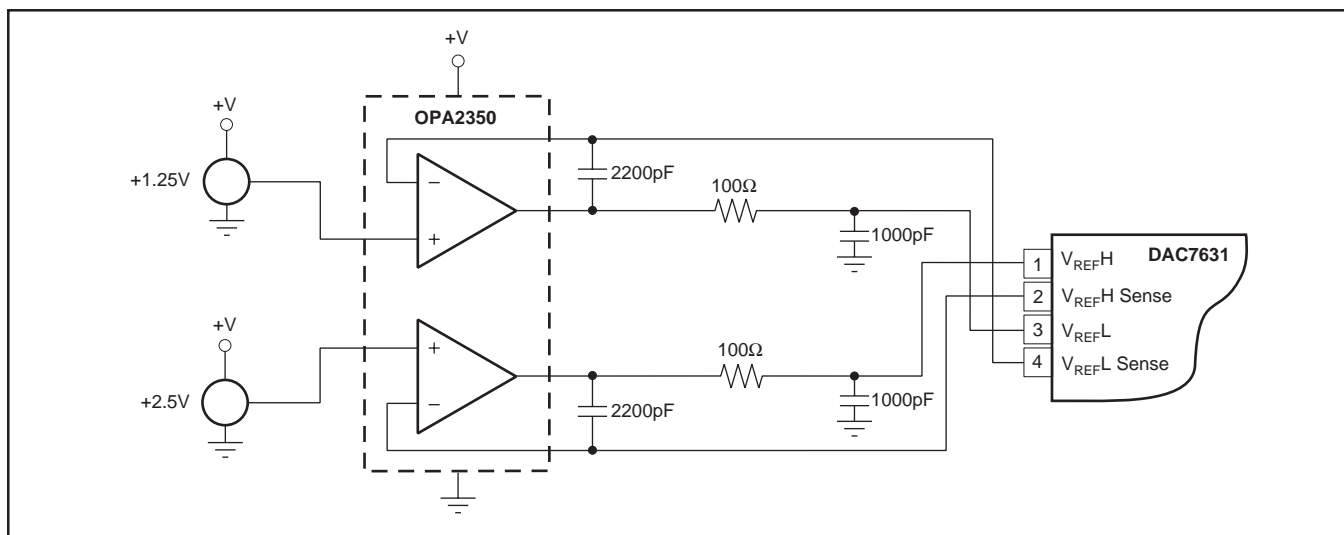
FIGURE 9. Single-supply Buffered Reference, V REFL = +1.25V, V REFH = -1.25V.
