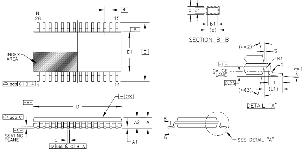
Package Number 360 - 28-Lead TSSOP, .173 Wide
