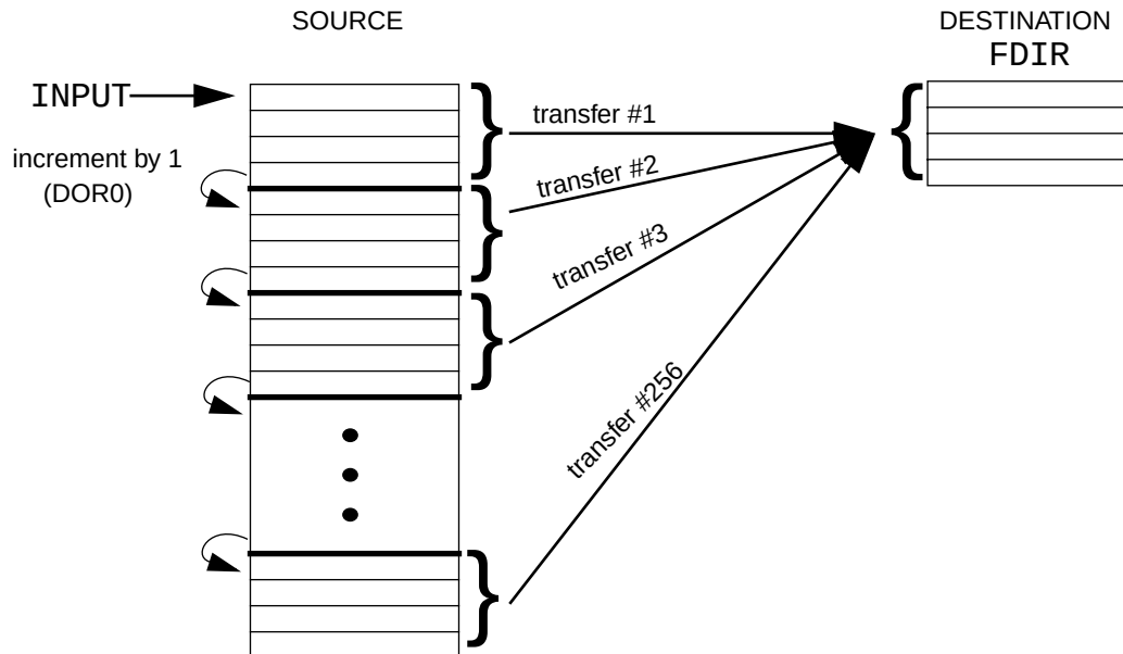
Figure 2-3. DMA Channel 0 Transfer
