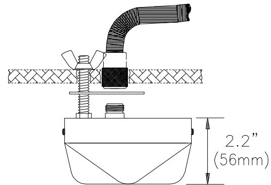
Ceiling Mount
