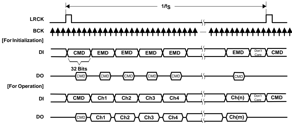
Figure 55. General TDMCA Frame
