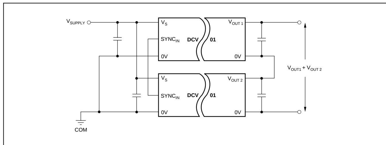
FIGURE 1. Connecting the DCV01 in Series.
