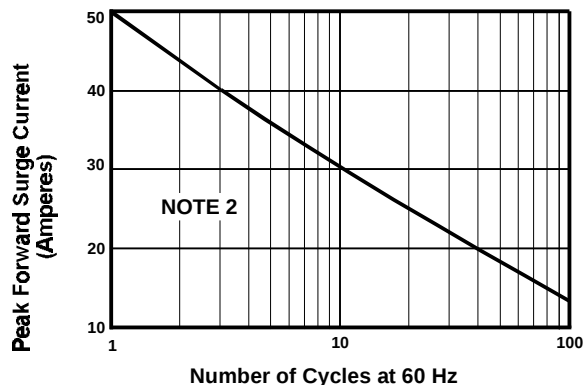
FIGURE 2. MAXIMUM NON-REPETITIVE SURGE CURRENT
