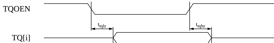
FIGURE 11. Synchronous Single-Port SRAM Test-Data Output-Enable Timing
