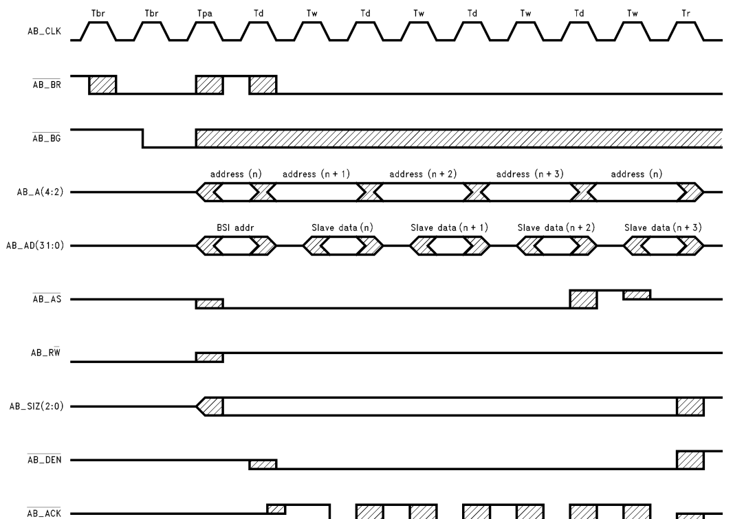
FIGURE 4-6. ABUS Burst Read, Physical Addressing, 16 Bytes, 1 W-S
