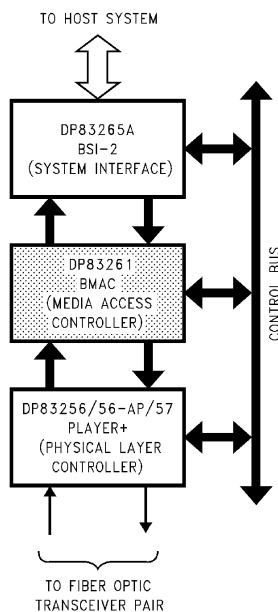
FIGURE 1-1. FDDI Chip Set Block Diagram
