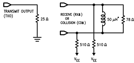
FIGURE 10. Test Loads
