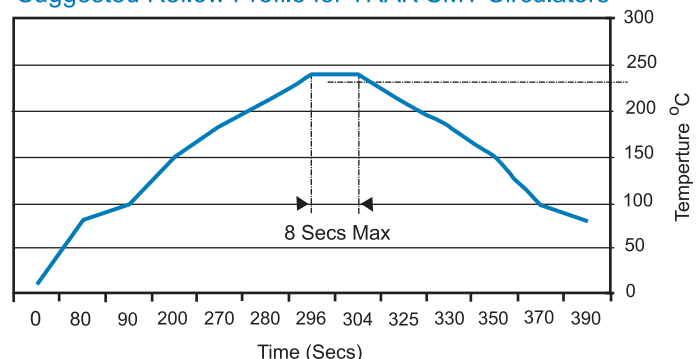
Suggested Reflow Profile for TRAK SMT Circulators
