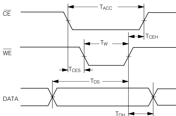
Figure 1. Timing Characteristics—Write Cycle Waveforms
