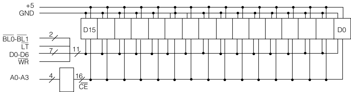
Figure 4. 16 Digits Interconnection
