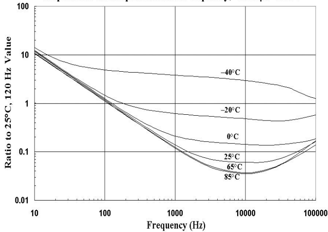
Impedance vs Temperature and Frequency, 4800 \mu F 200 V
