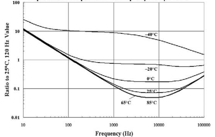
Impedance vs Temperature and Frequency 7900 \mu F 400 V
