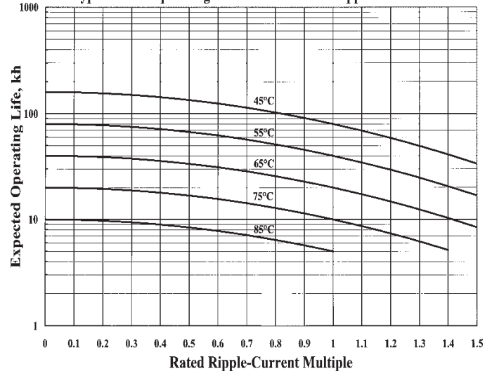
Type DCMC Operating Life in Kilohours vs Ripple Current
