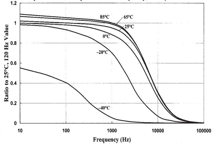
Capacitance vs Temperature and Frequency, 7900 \mu F 400 V
