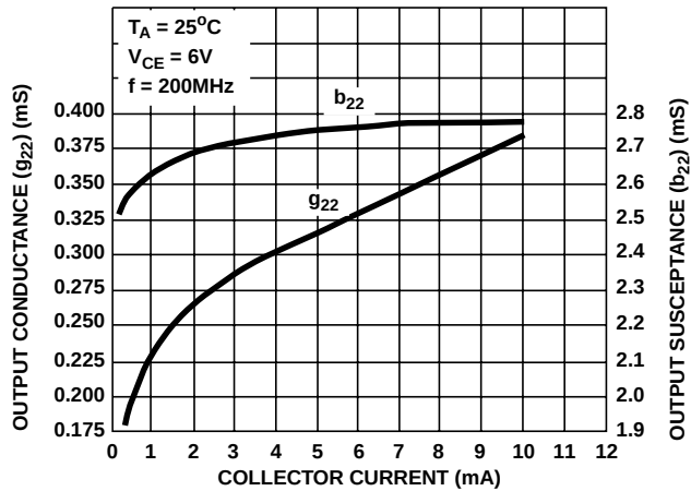
FIGURE 15. OUTPUT ADMITTANCE ( Y_{22} ) vs COLLECTOR CURRENT
