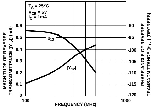
FIGURE 19. REVERSE TRANSADMITTANCE ( Y_{12} ) vs FREQUENCY
