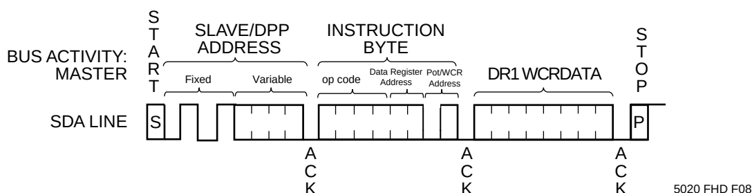
Figure 6. Write Timing
