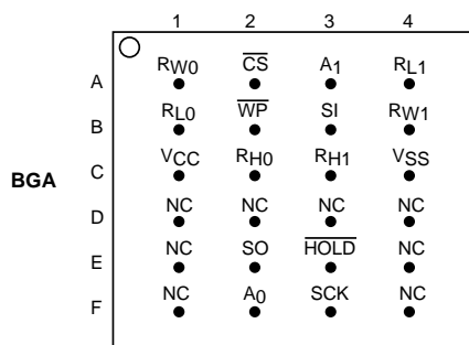
Top View - Bump Side Down
