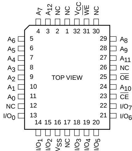
PLCC Package (N)
