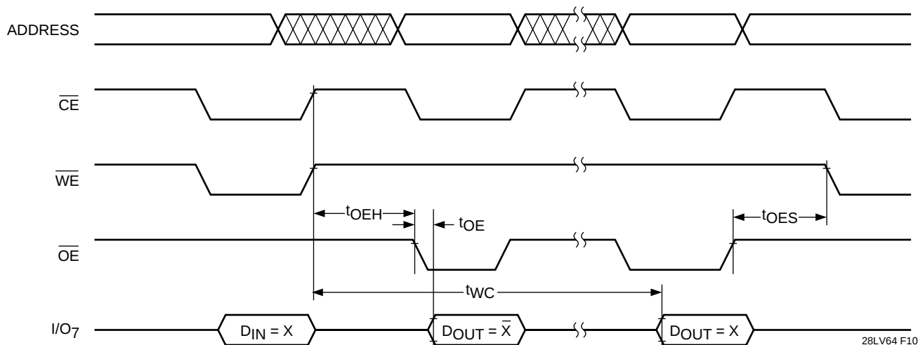
Figure 7. DATA Polling
