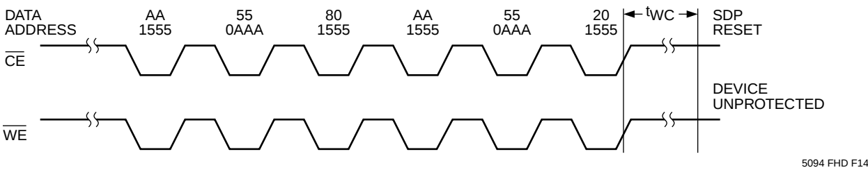
Figure 12. Resetting Software Data Protection Timing
